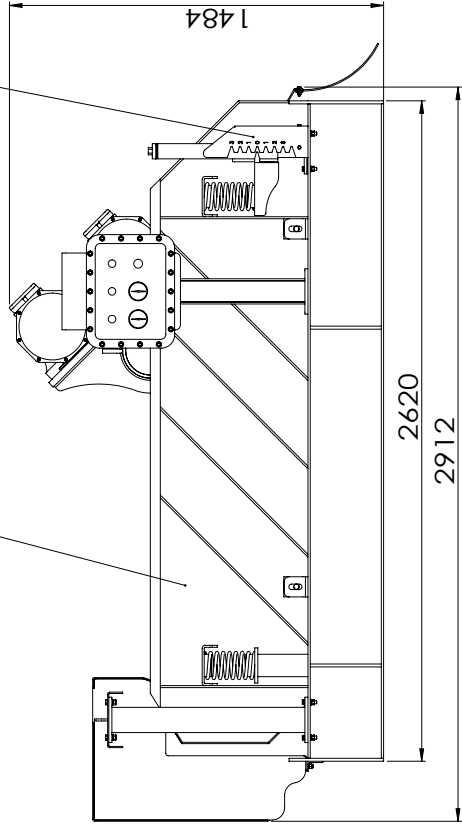
ELEVATION VIEW
